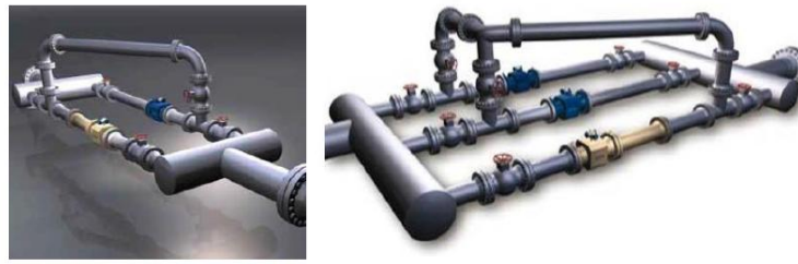
Figure 2-2: Z configuration
