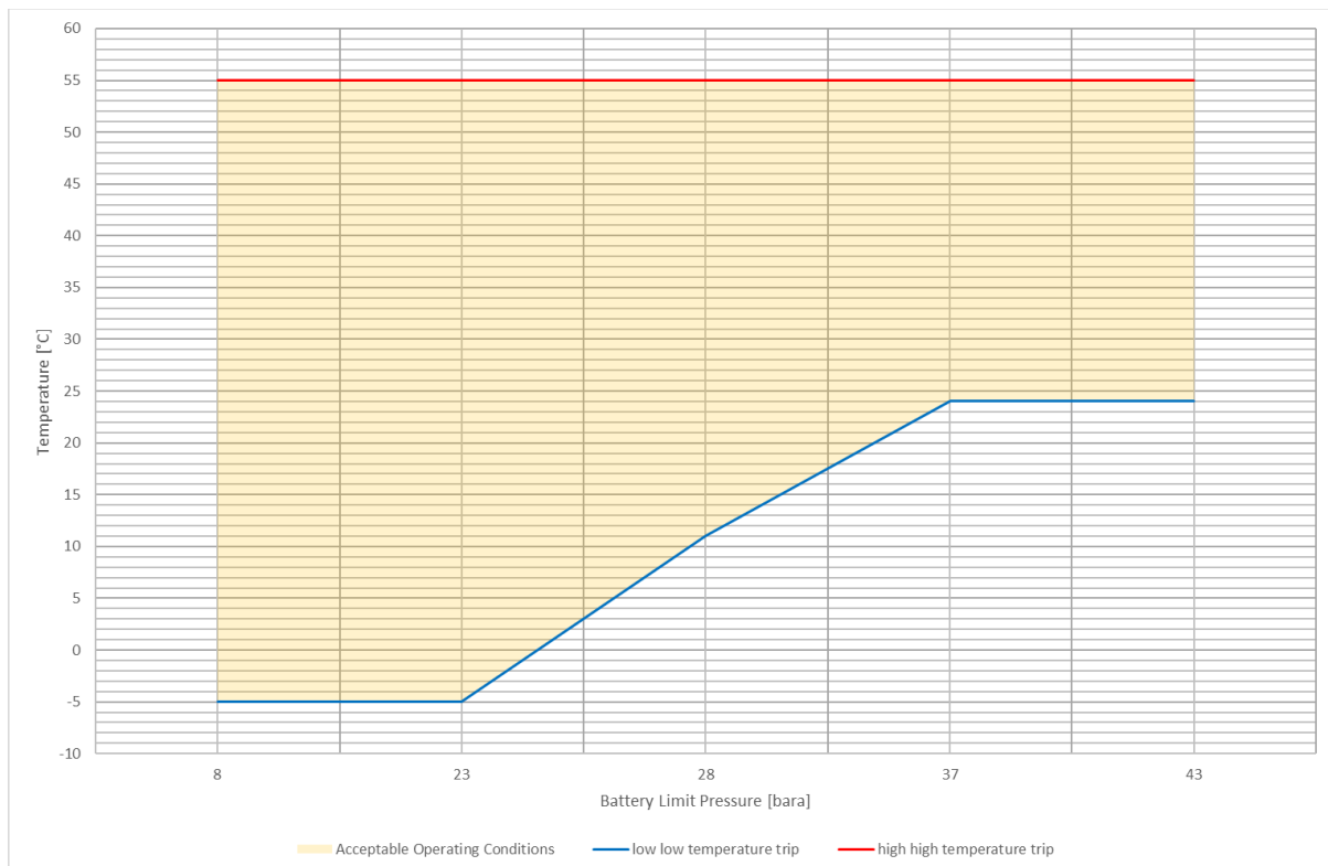
Figure 1-1: entry conditions at the Battery Limits
